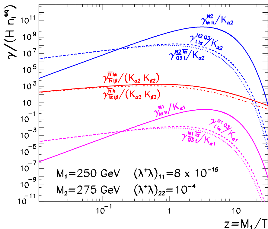
Figure 2. Reaction densities included in the Boltzmann equations as a function of z = M_1/T , normalized to H n_\ell^{eq} , where H is the expansion rate of the universe.
