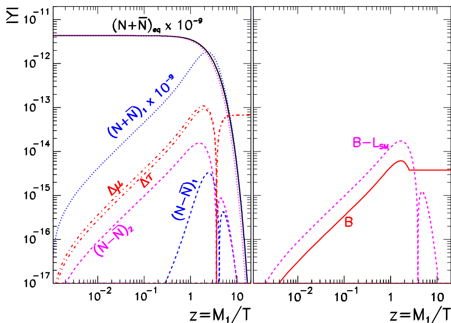
Figure 4. The asymmetries |Y_{\Delta_\alpha}| , |Y_{N_i-\bar{N}_i}| , Y_{B-L_{SM}} , and the densities Y_{N_i+\bar{N}_i} , Y_{N_i+\bar{N}_i}^{eq} as a function of z for the values of the parameters given in eq. (4.2). Note that the densities Y_{N_i+\bar{N}_i} and Y_{N_i+\bar{N}_i}^{eq} have been rescaled by 10^{-9} in order to fit into the figure.
