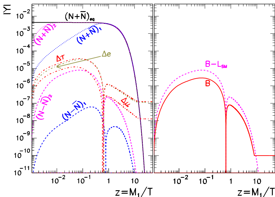
Figure 3. The asymmetries |Y_{\Delta_\alpha}|, |Y_{N_i-\bar{N}_i}|, Y_{B-L_{SM}} , and the densities Y_{N_i+\bar{N}_i}, Y_{N_i+\bar{N}_i}^{eq} as a function of z for the values of the parameters given in eq. (4.1).
